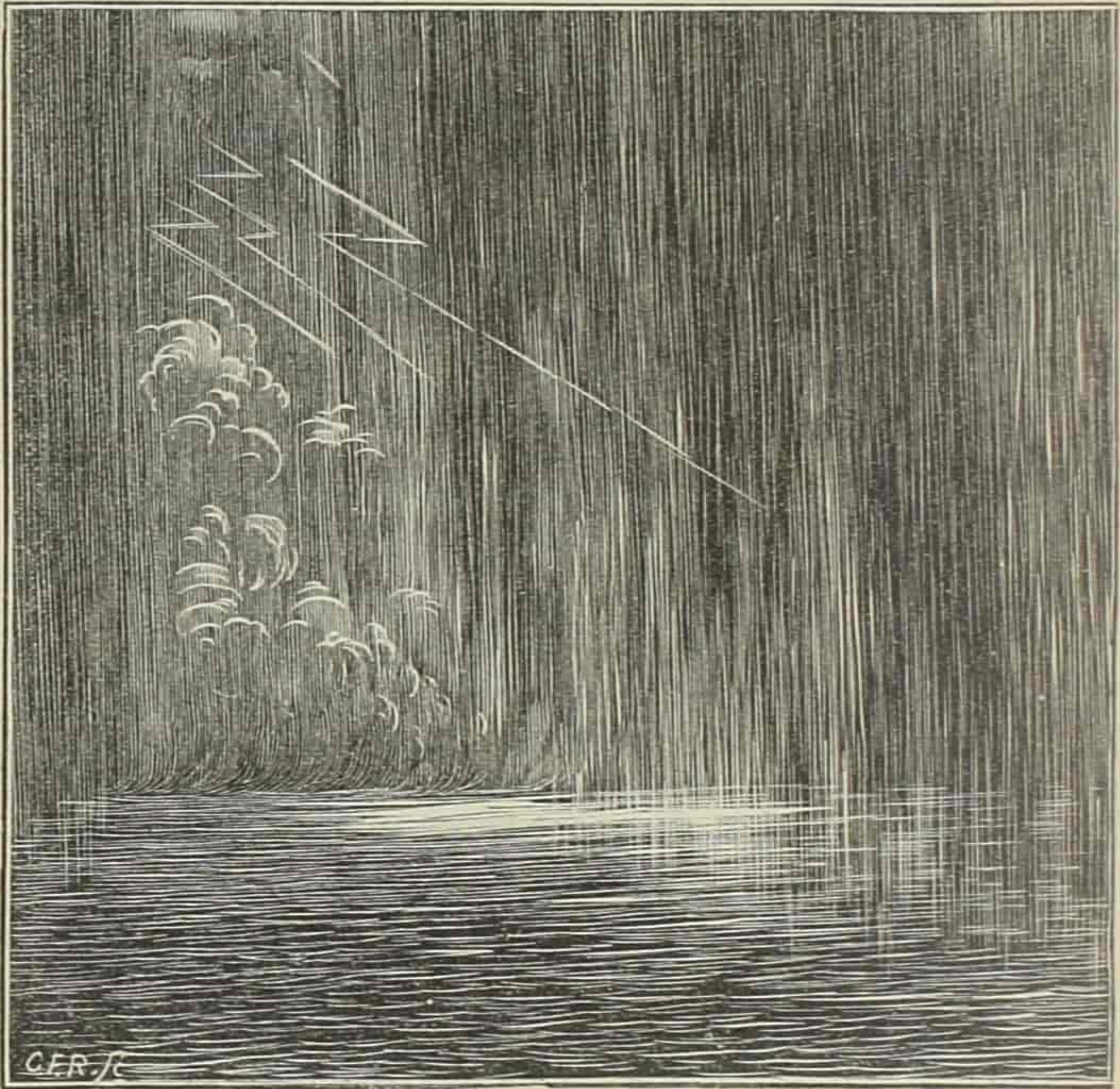
THE PRIMEVAL STORM.
