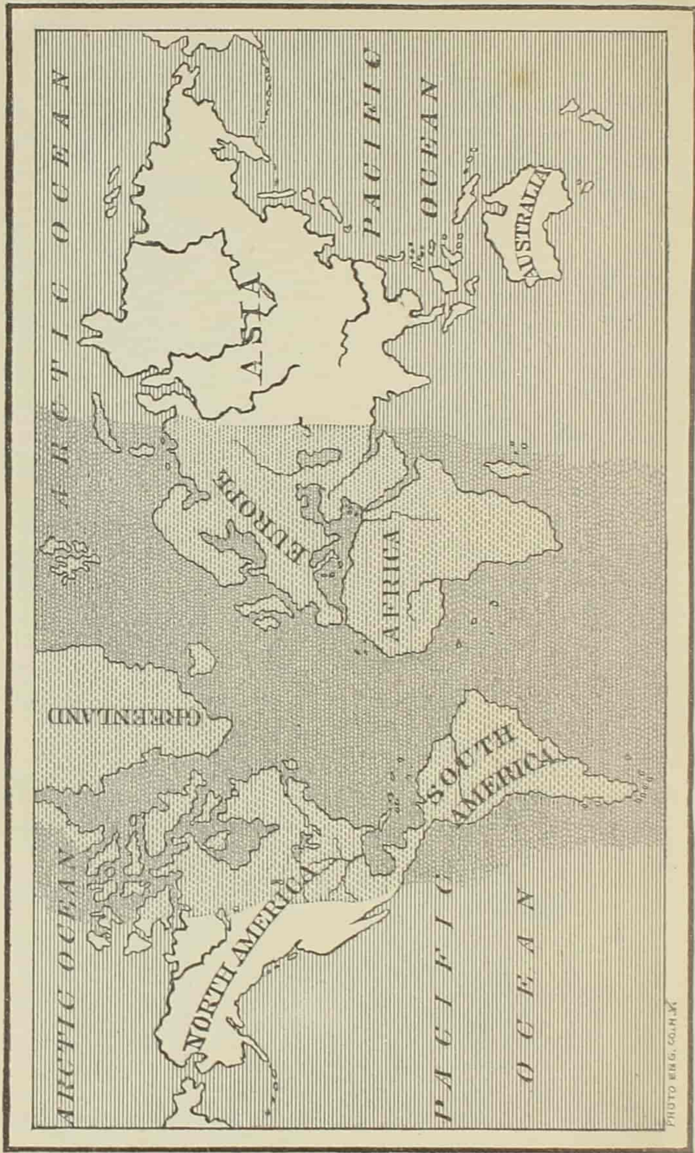
THE GEOGRAPHICAL DISTRIBUTION OF THE DRIFT.
