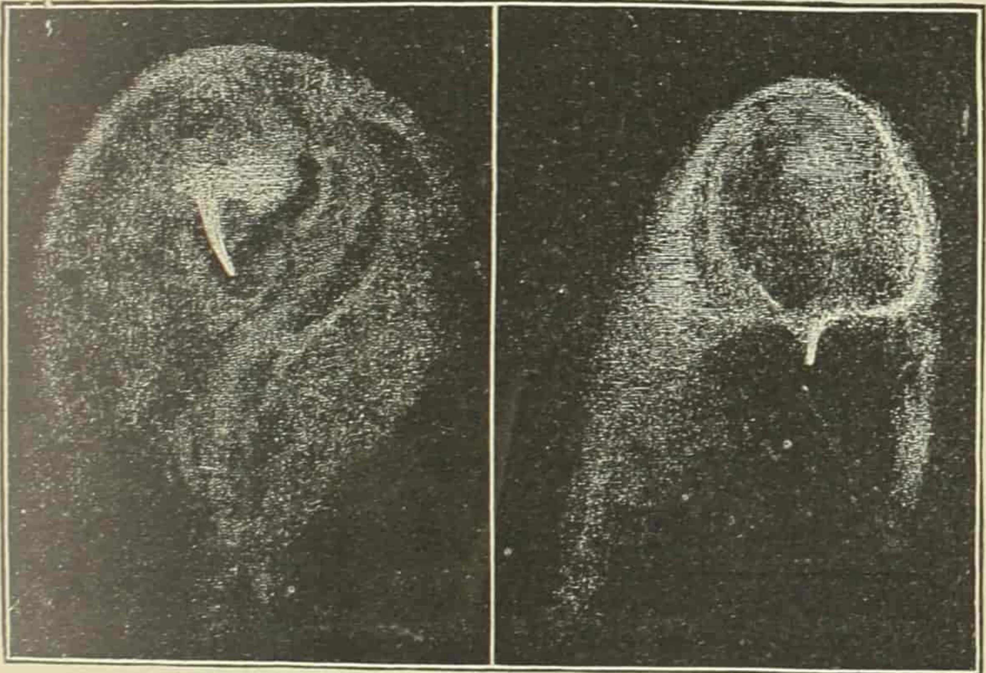
COMET OF 1862.
