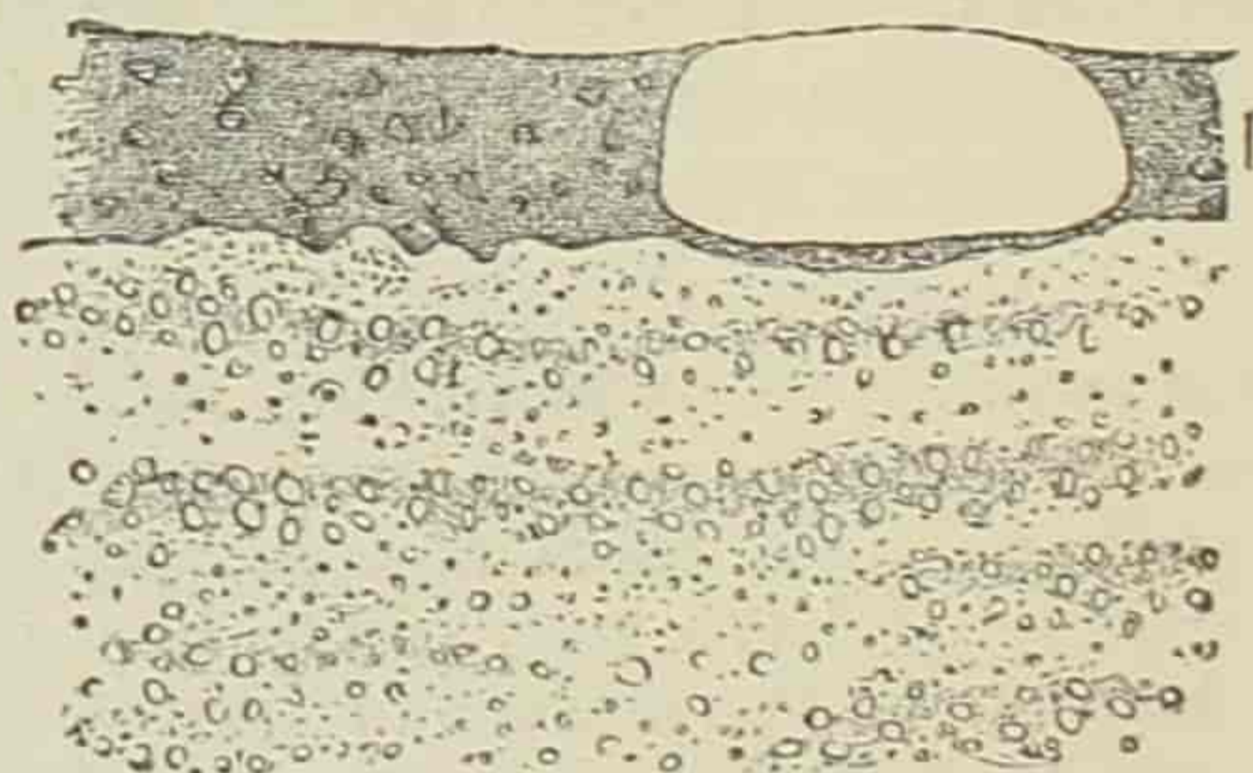
SECTION AT JOINVILLE.
