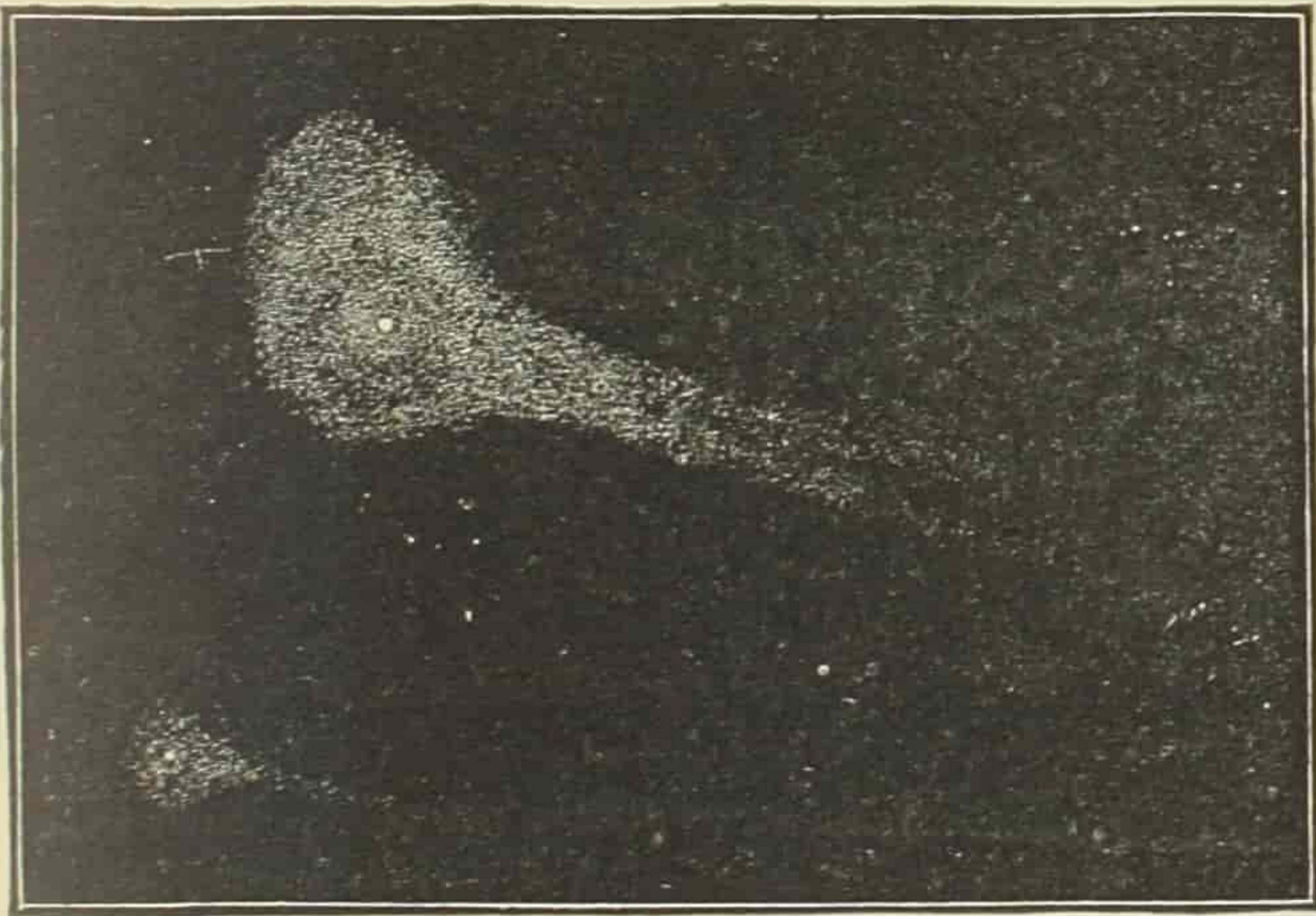
BIELA'S COMET, SPLIT IN TWO.
