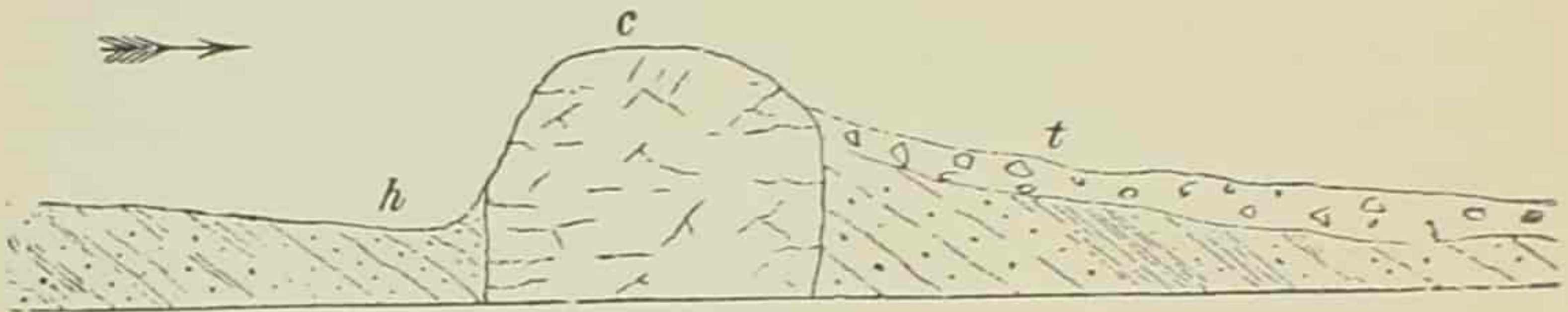
CRAG AND TAIL.— c , crag ; t , till.
