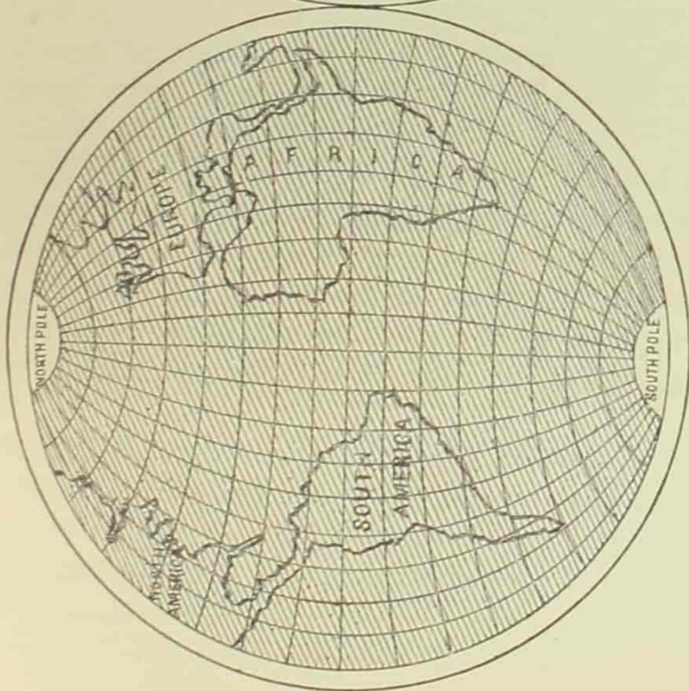
THE SIDE OF THE EARTH STRUCK BY THE COMET.
