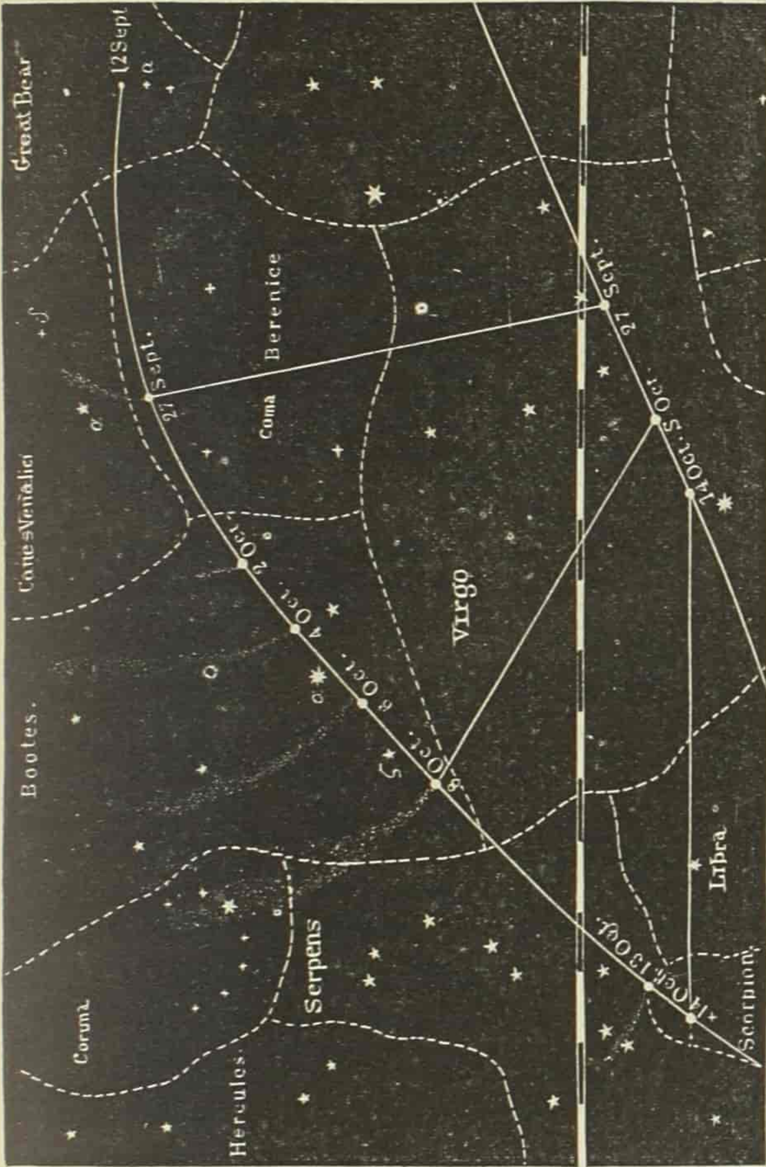
COURSE OF DONATI'S COMET.
