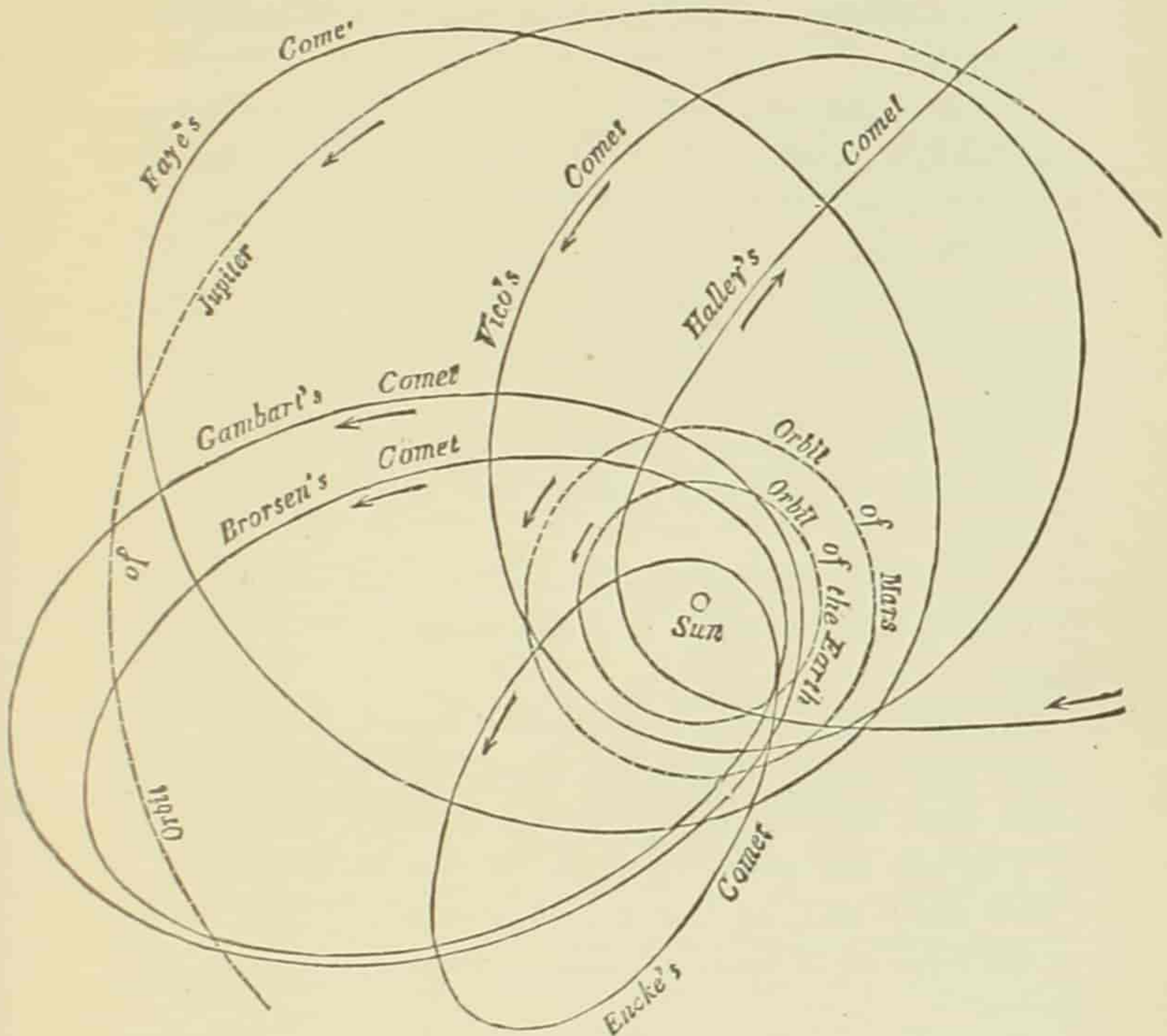
ORBITS OF THE PERIODIC COMETS.
