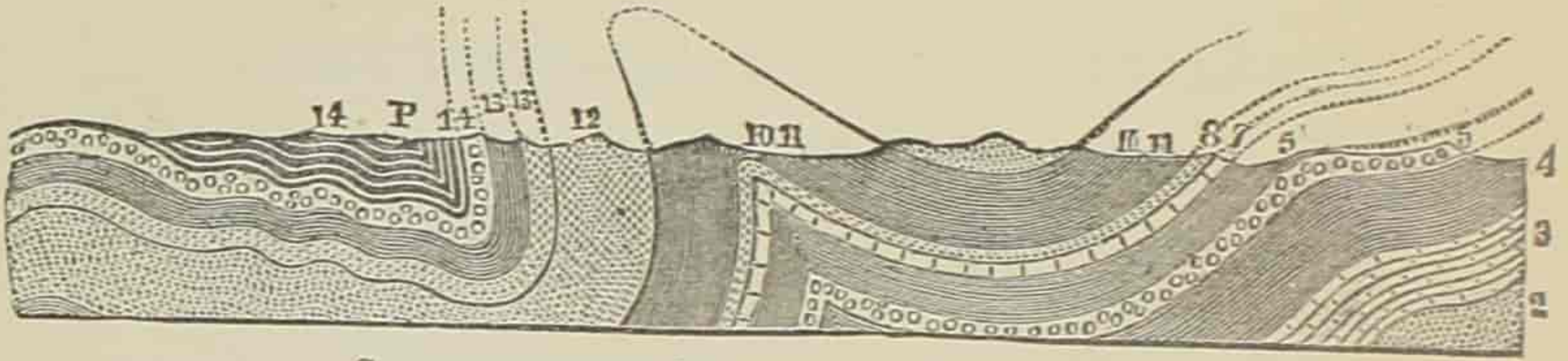
SECTION ON THE SCHUYLKILL, PENNSYLVANIA.
