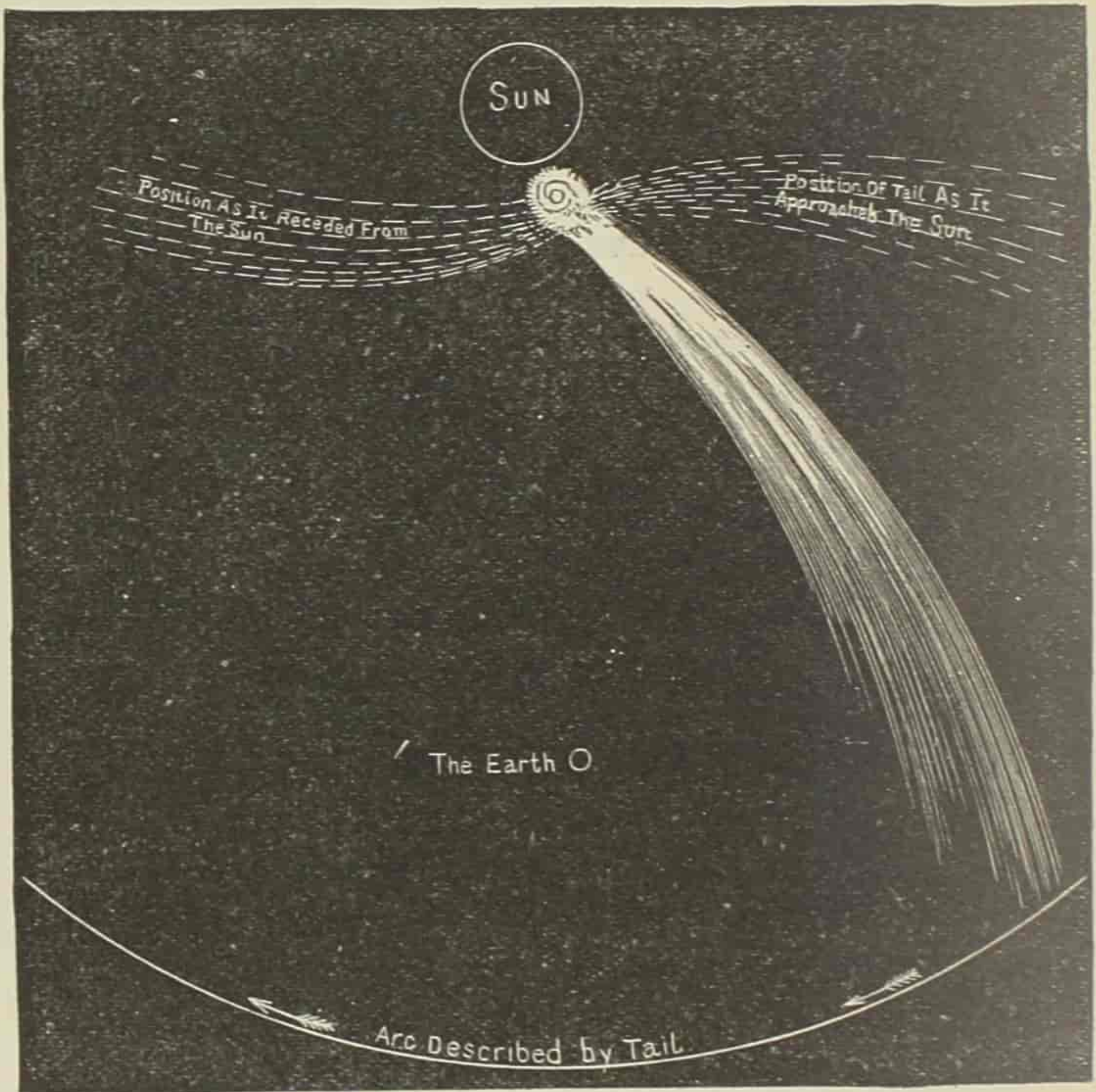
THE COMET SWEEPING PAST THE EARTH.
