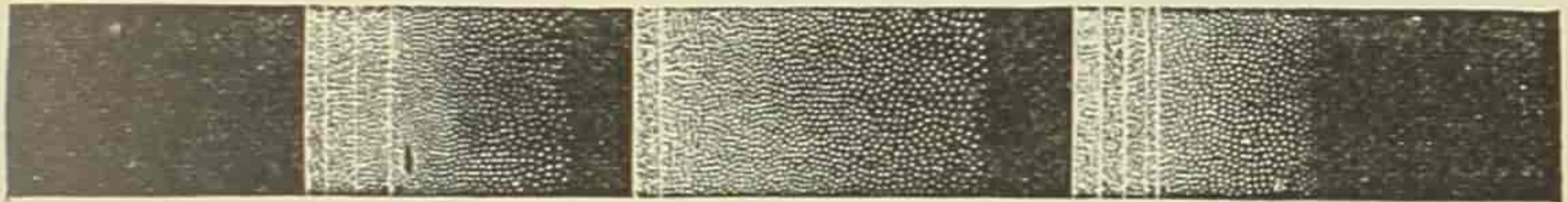
Spectrum of Carbon in Olefiant Gas.
