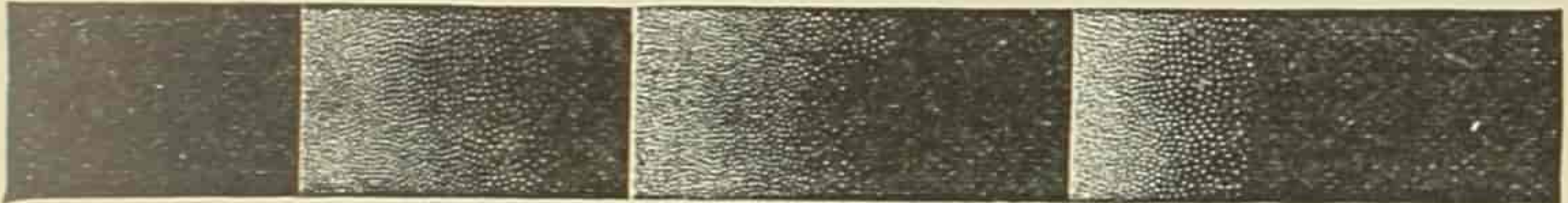
Winnecke's Comet II. 1868.
