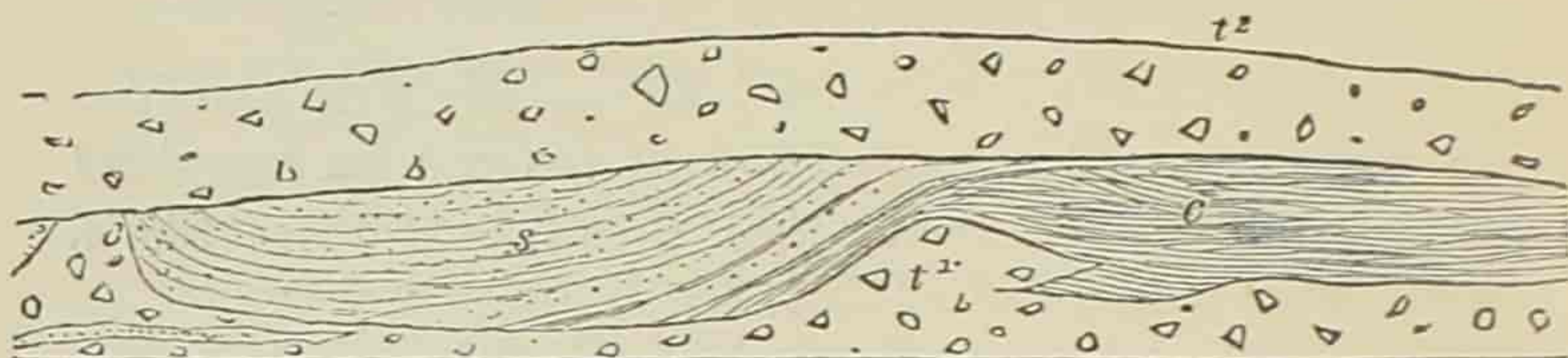
STRATIFIED BEDS IN TILL, LEITHEN WATER, PEEBLESSHIRE, SCOTLAND.
