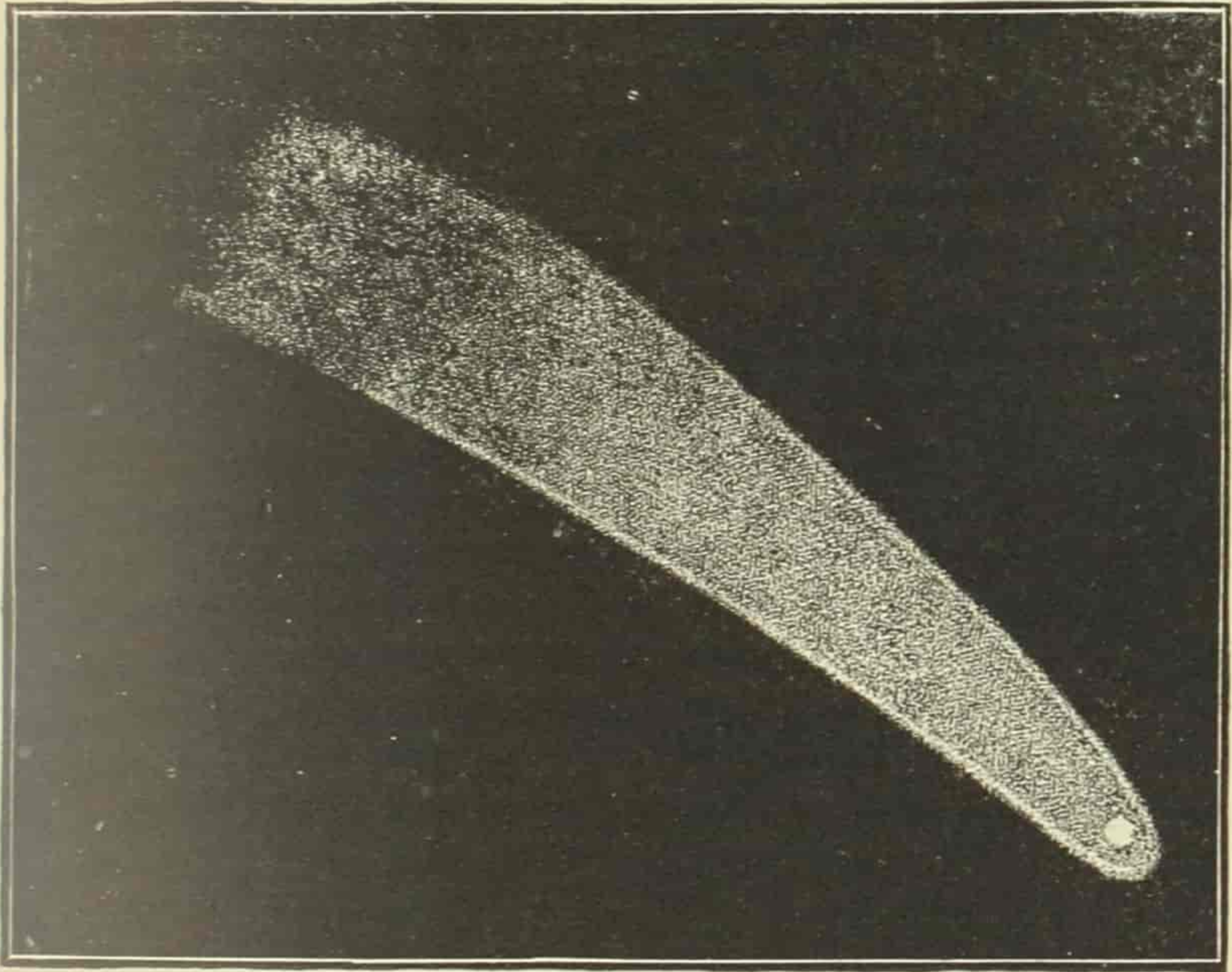
THE GREAT COMET OF 1811.
