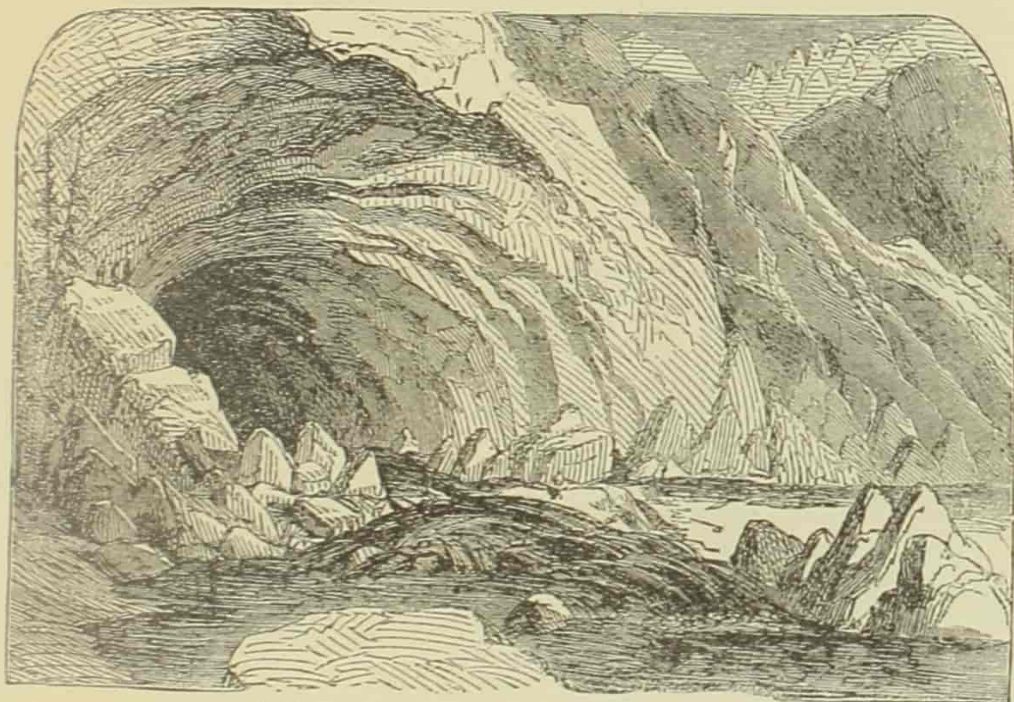
A RIVER ISSUING FROM A SWISS GLACIER.
