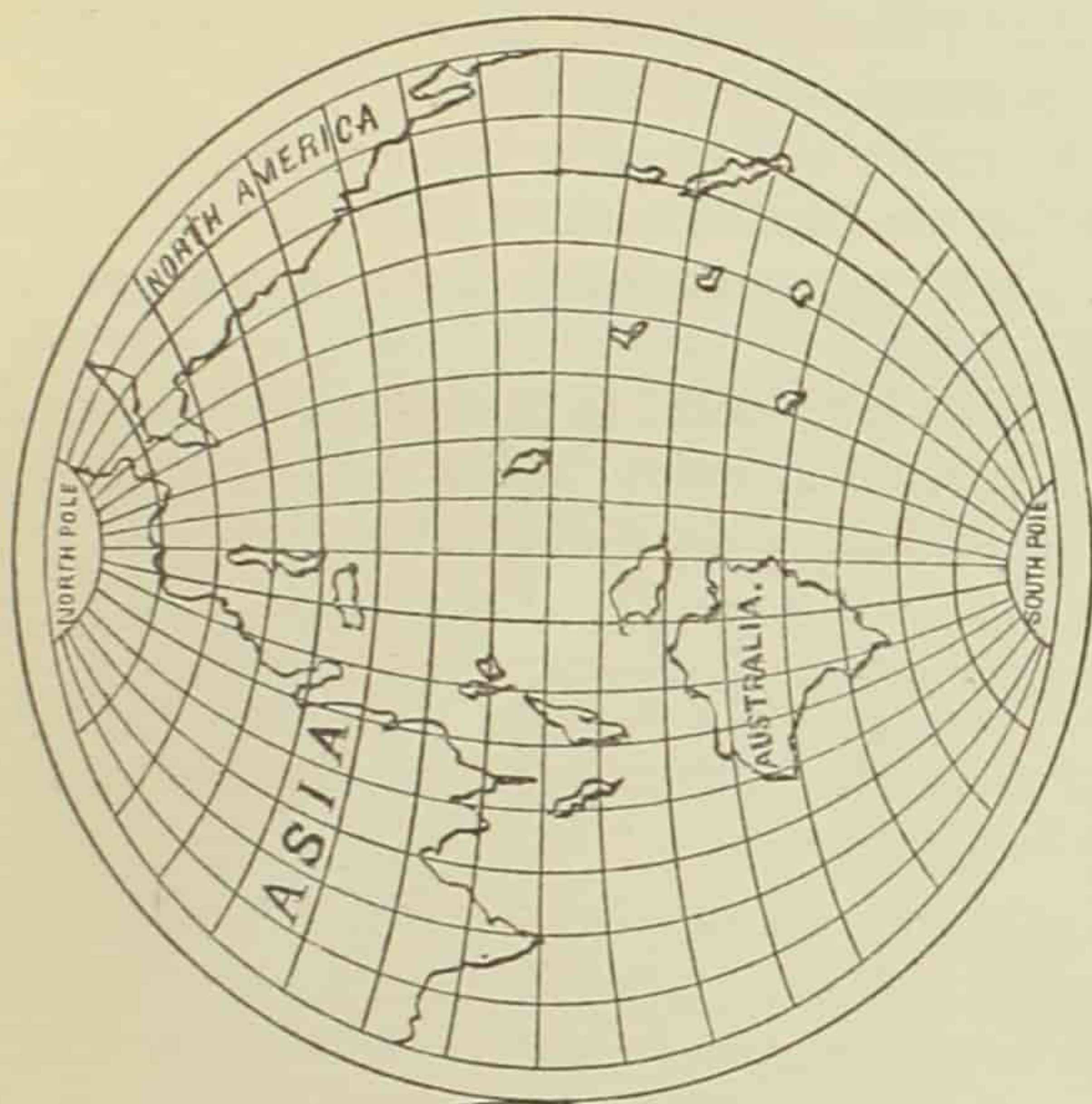
THE SIDE NOT STRUCK BY THE COMET.
