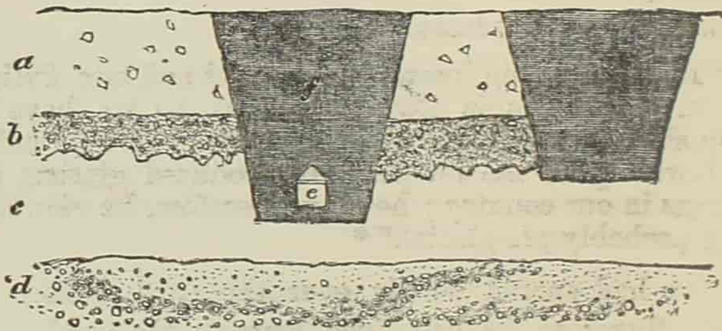
SECTION AT ST. ACHEUL.
