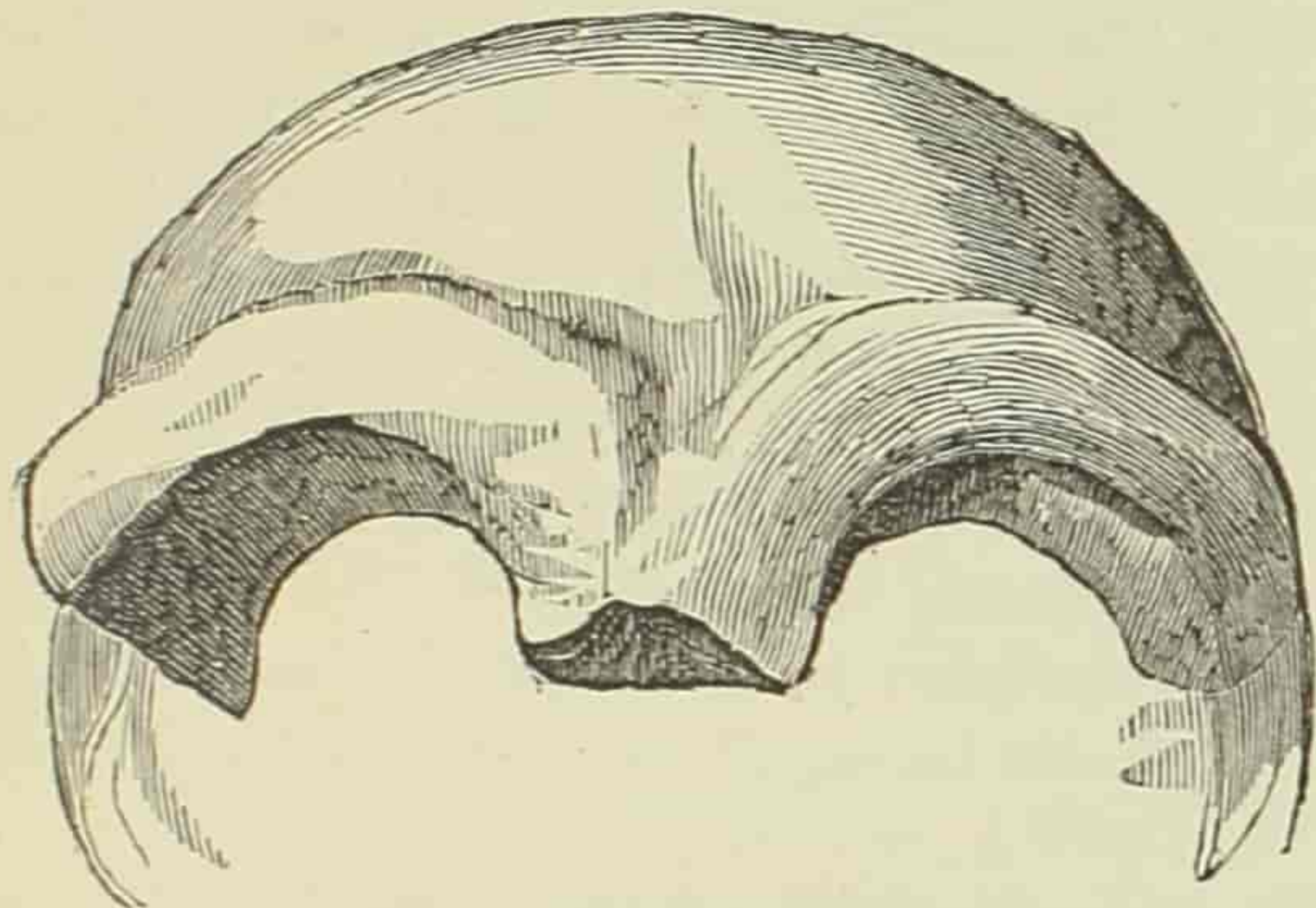
THE NEANDERTHAL SKULL.
