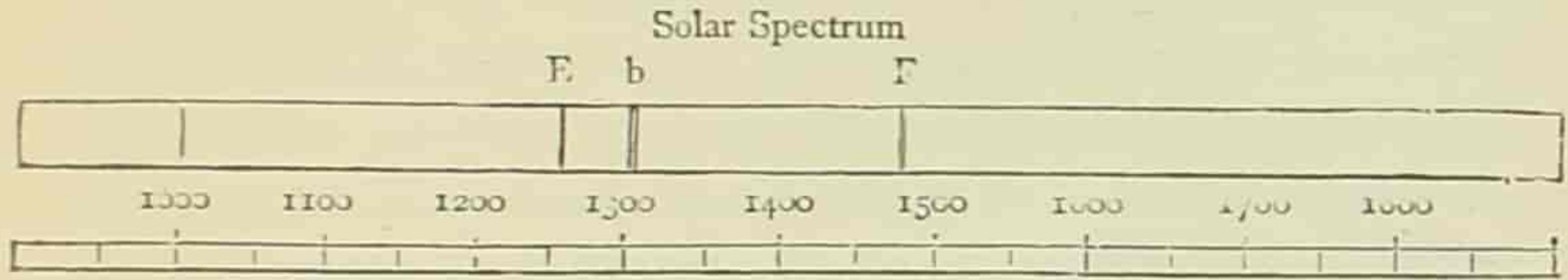
Spectrum of Carbon in Olive-Oil.
