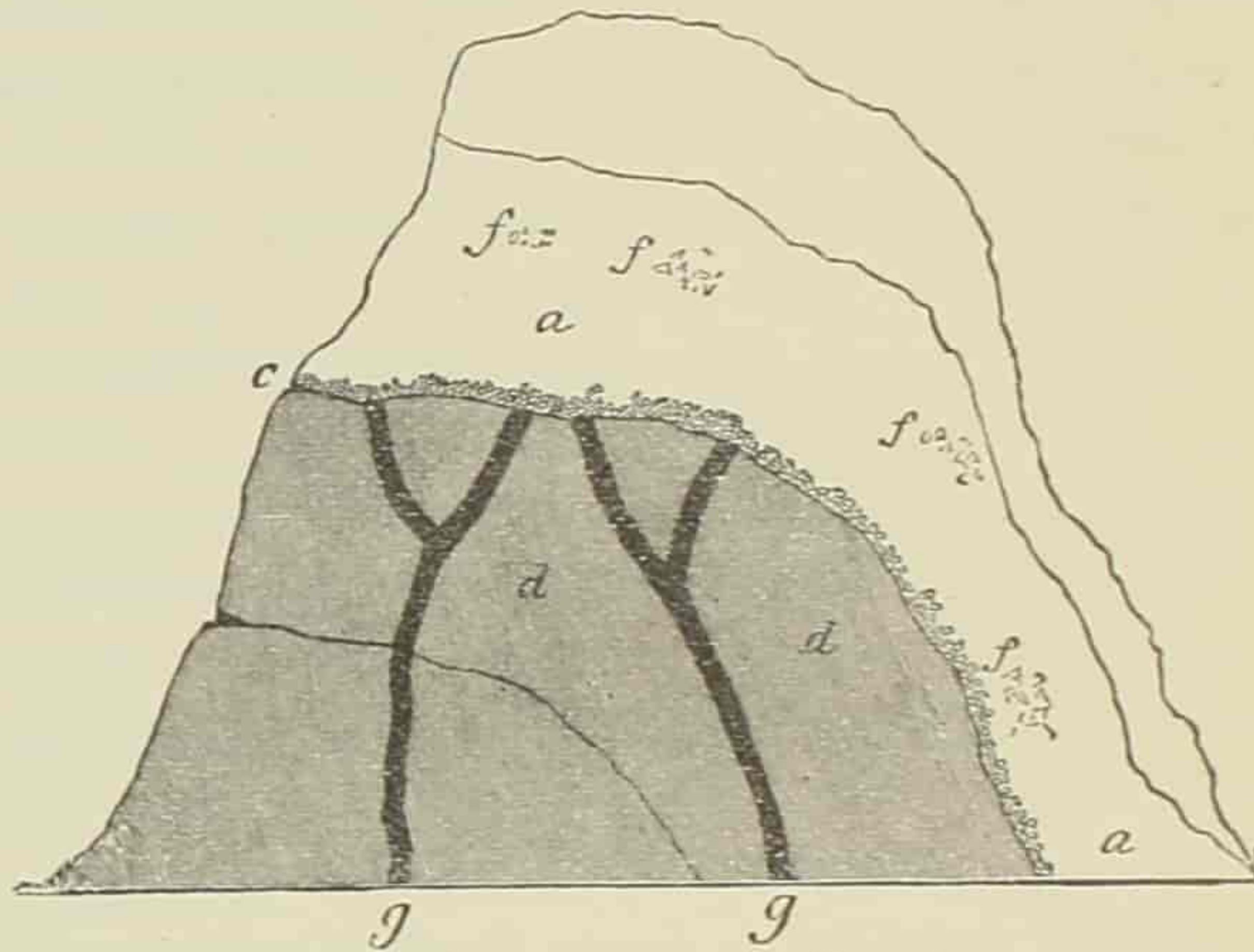
DRIFT-DEPOSITS IN THE TROPICS.
